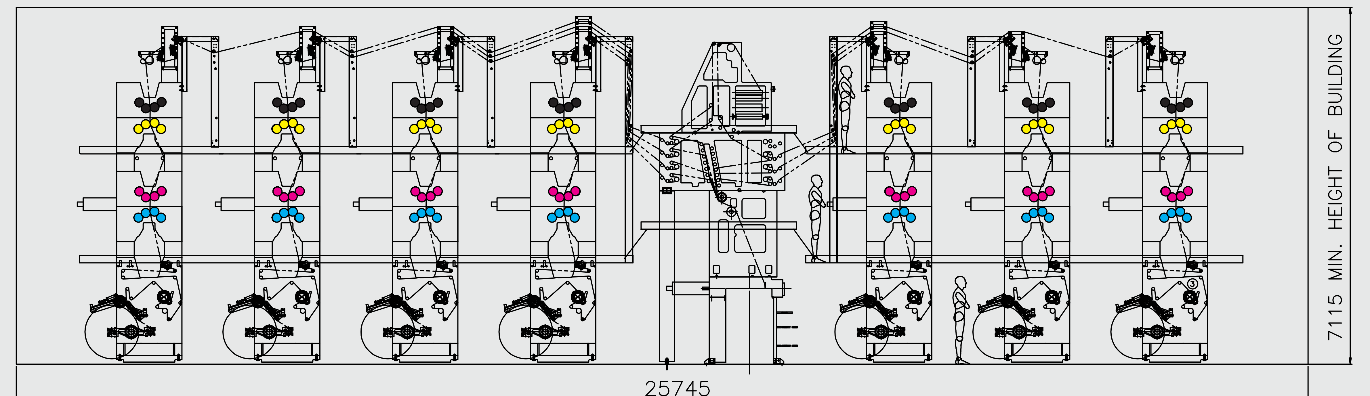
CITYLINE EXPRESS TOWER WITH INTEGRATED AUTOPASTER AT M/S JAGRAN PRAKASHAN, RANCHI, INDIA
