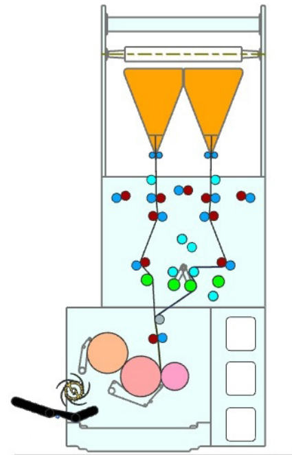
Jaw Folder 2:3:3 (Single Delivery)
