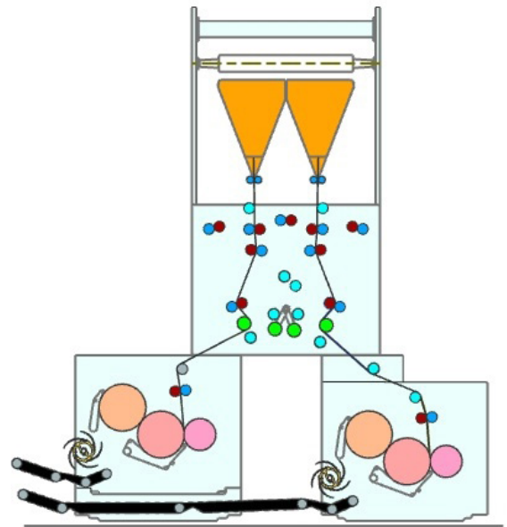
Jaw Folder 2:3:3 (Double Delivery)
